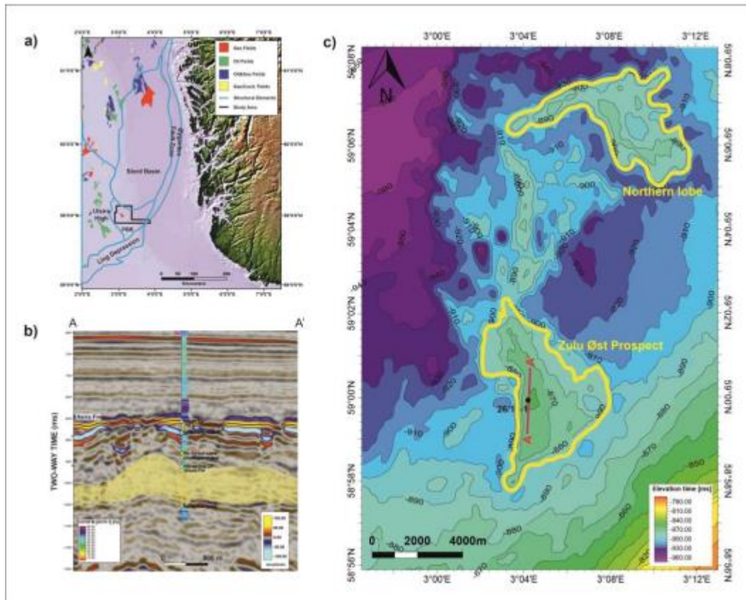
Figure 1 a) Location of the study area. Figure made with GeoMapApp ( www.geomapp.org ) using Norwegian Petroleum Directorate database. b) Seismic sections at the well location of Zulu Øst field c) Two-way-time map of Top Utsira Formation showing Zulu Øst Field and northern lobe.
