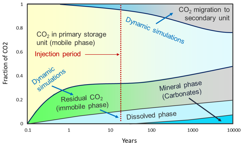
Sketch illustrating the likely short- and long-term fate of CO 2 in the storage complex with the main CO 2 trapping mechanisms (modified from Ringrose and Bentley 2021)
